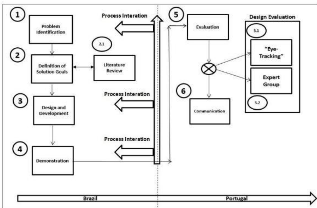
Figure 1: Methodological Flow
